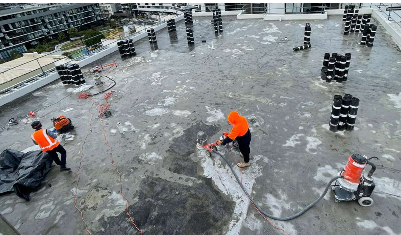
Cleaning and Removing of Existing Membrane
